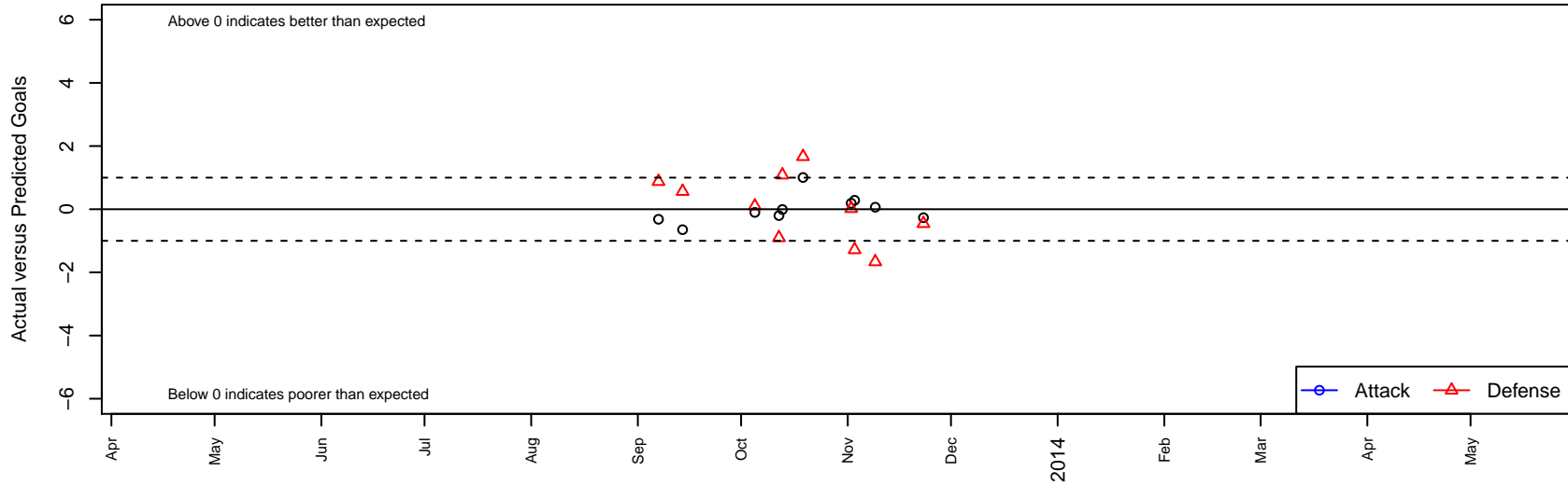
BUSC 01 Premier B00 Dots are actual minus expected GF (blue circles) and GA (red triangles). Blue line is smoothed change in attack strength. Red is smoothed change in defense strength.
